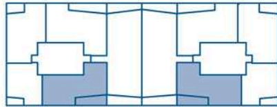
LEVELS 09-20
